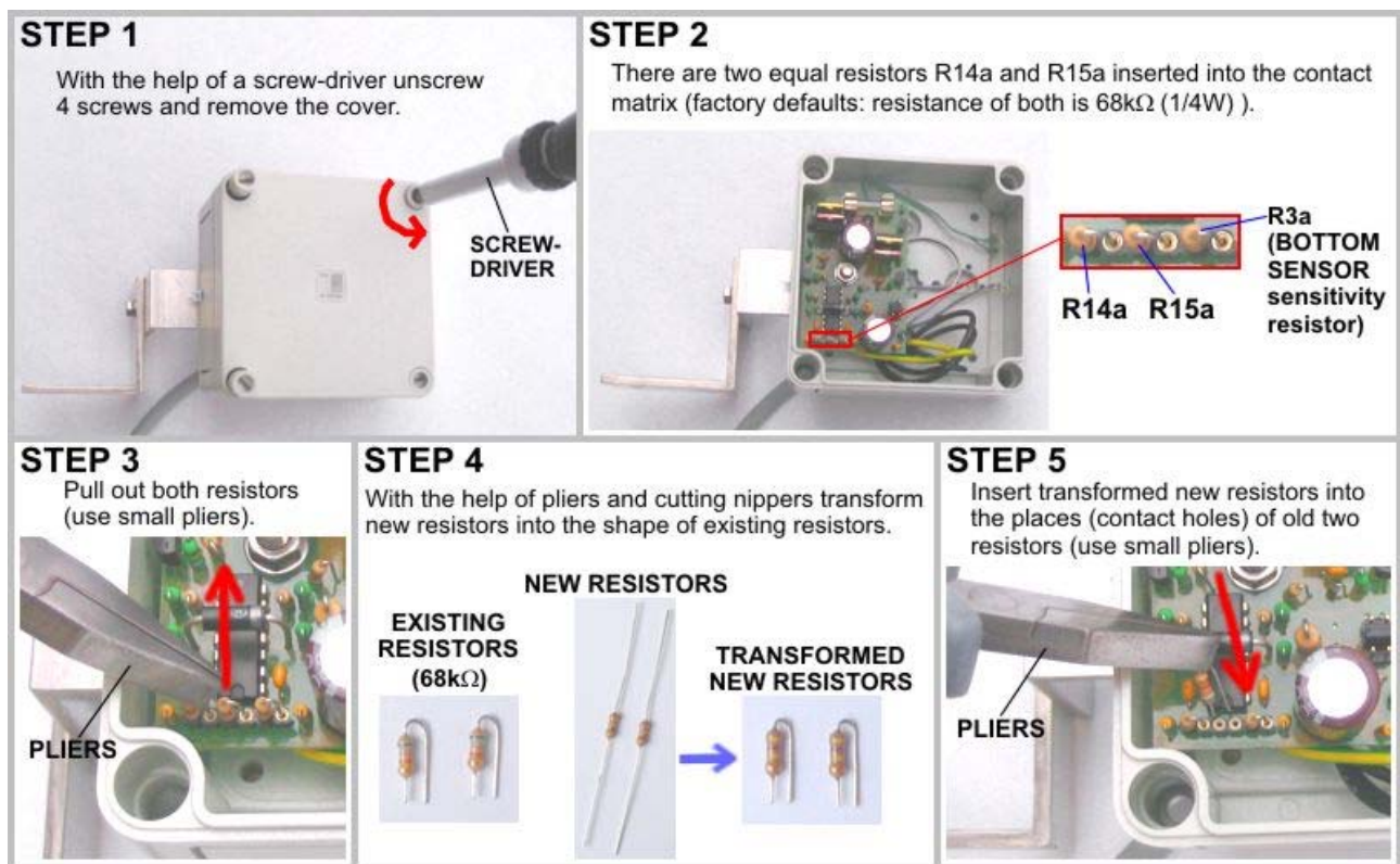
Figure 5: Changing the tracking accuracy (changing R14a and R15a)
