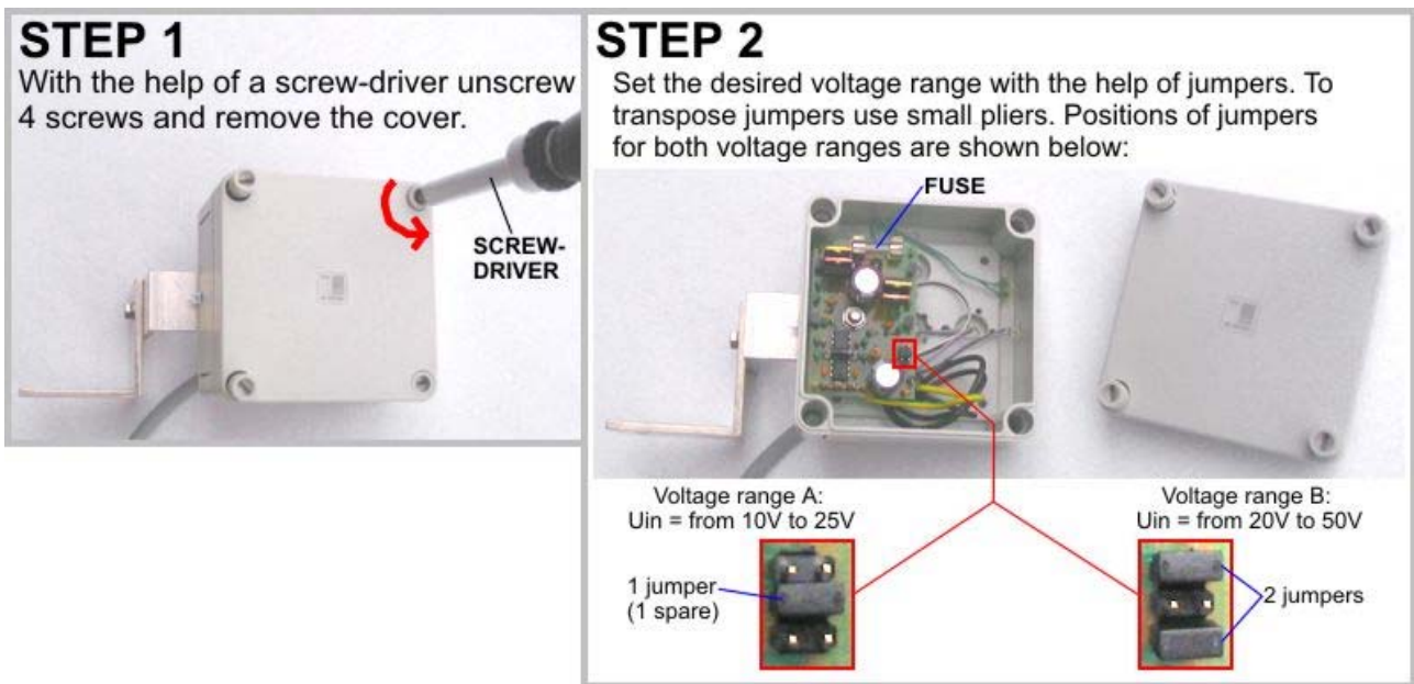
Figure 2: Setting the input voltage range
