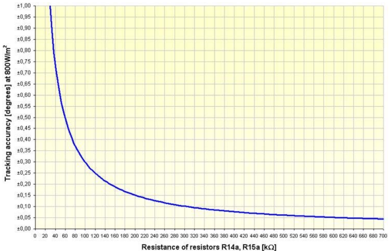
Figure 4: How tracking accuracy depends on different resistance of resistors R14a and R15a at solar irradiance of 800W/m 2
