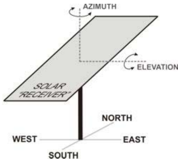
Figure 7: Dual-axis tracking (shown for northern hemisphere)
