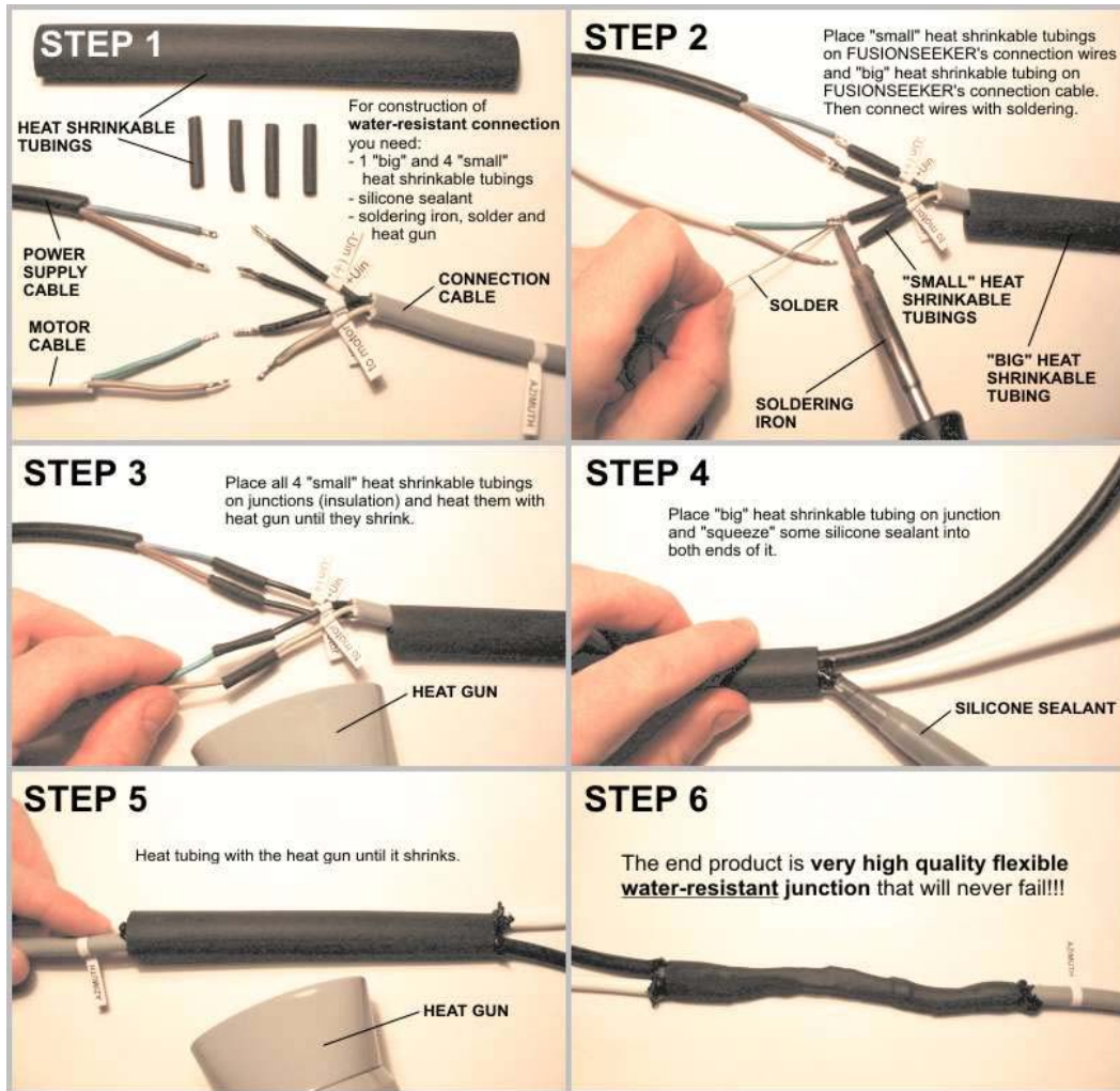
Figure 10: "Joining" "azimuth" or "elevation" connection cable with its power supply cable and motor cable
