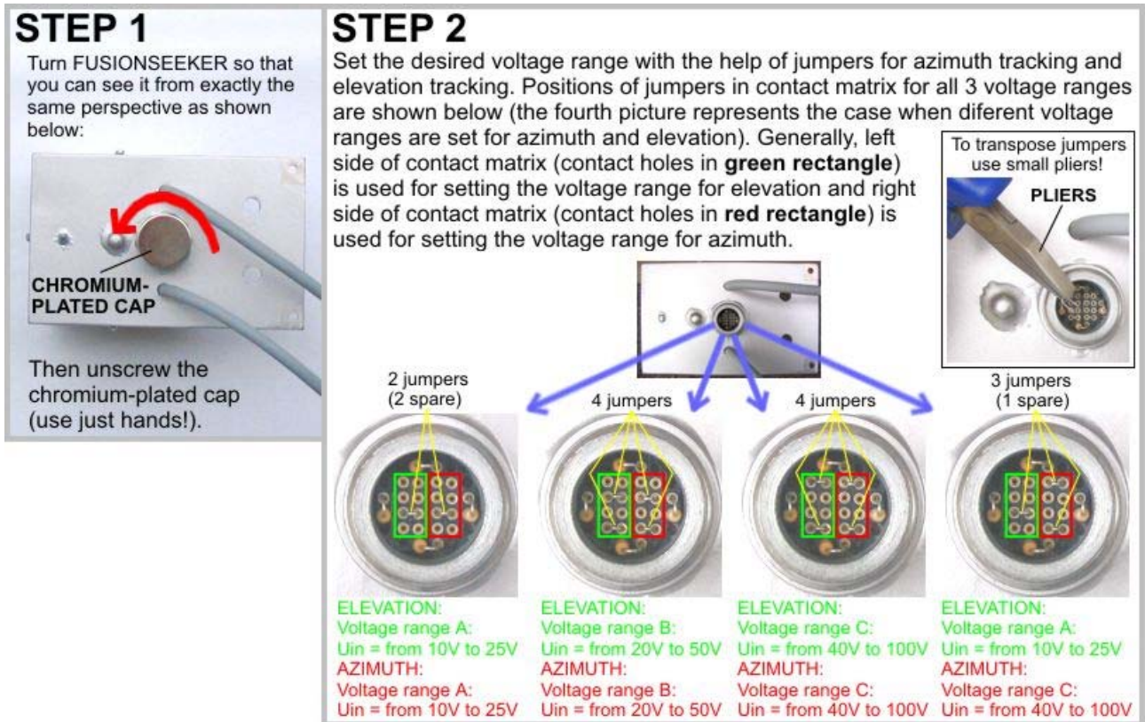
Figure 3: Setting the input voltage range
