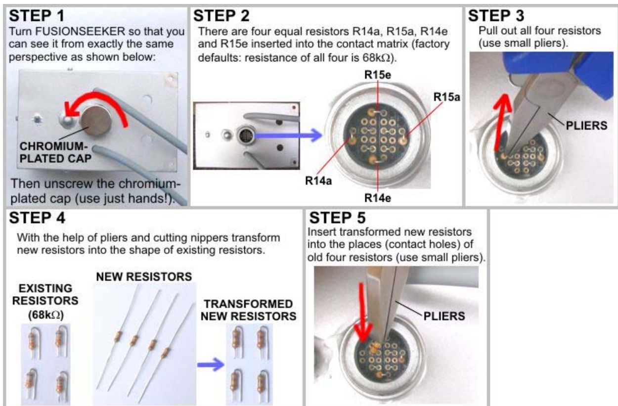
Figure 6: Changing the tracking accuracy (changing R14a, R15a, R14e and R15e)
