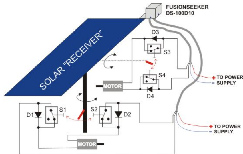
Figure 12: Installing the limit switches
