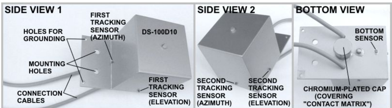
Figure 2: Components of FUSIONSEEKER DS-100D10
