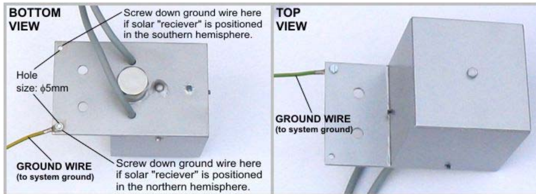
Figure 14: Grounding the FUSIONSEEKER DS-100D10
