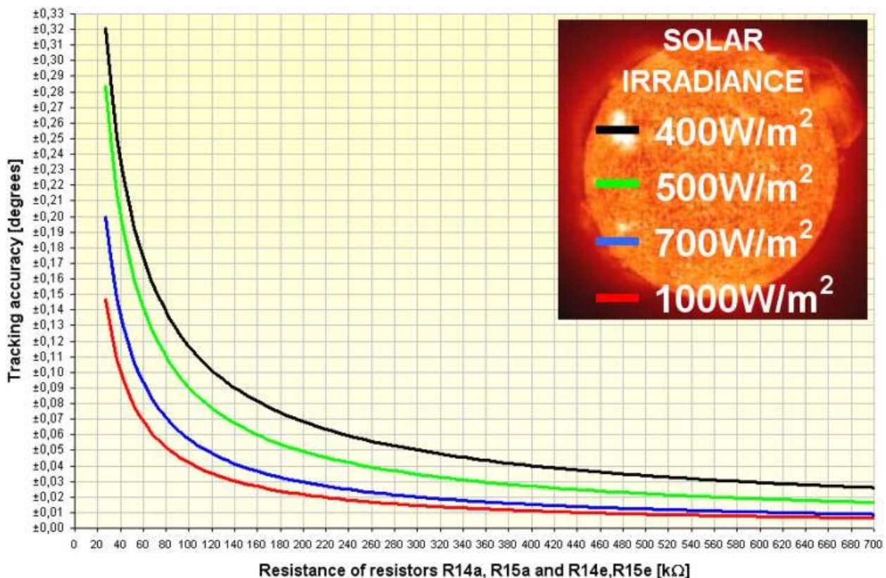
Figure 5: How tracking accuracy depends on different resistance of resistors R14a, R15a, R14e and R15e at certain solar irradiance
